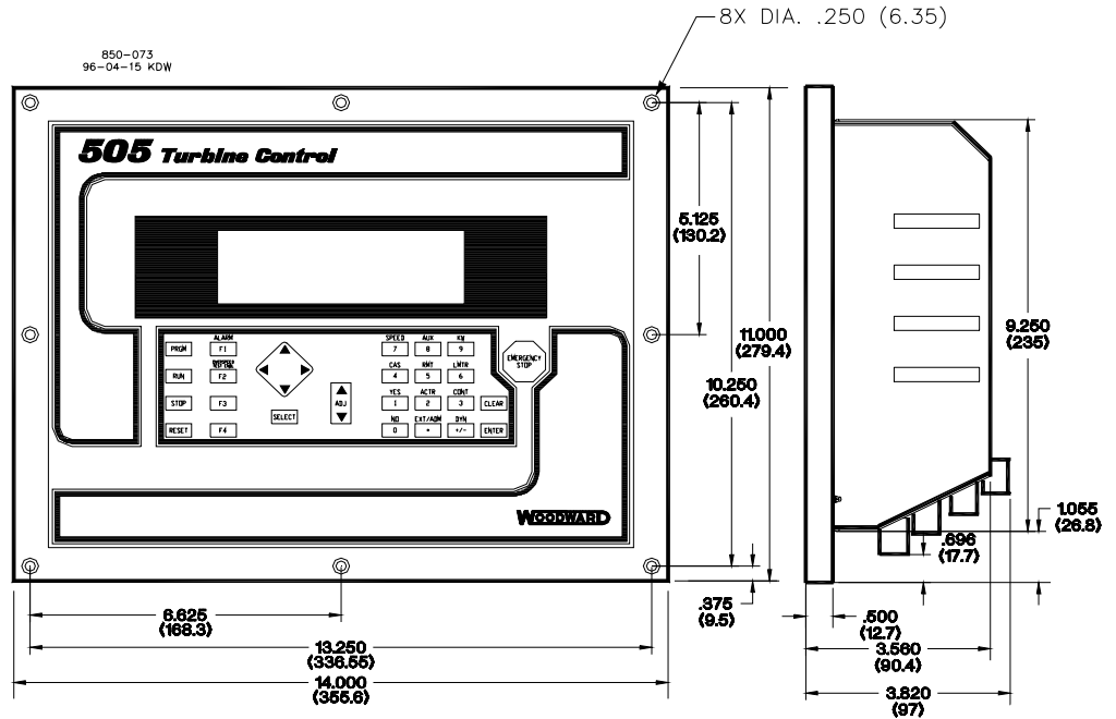
505/505E Dimensions (Do not use for construction)
