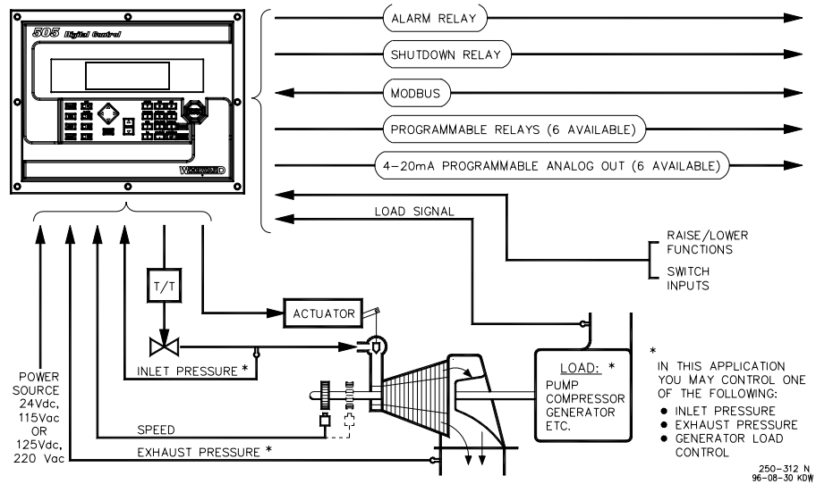
Controlled Single Valve Steam Turbine
