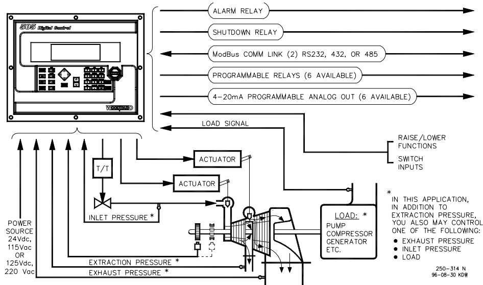
Controlled Extraction Steam Turbine
